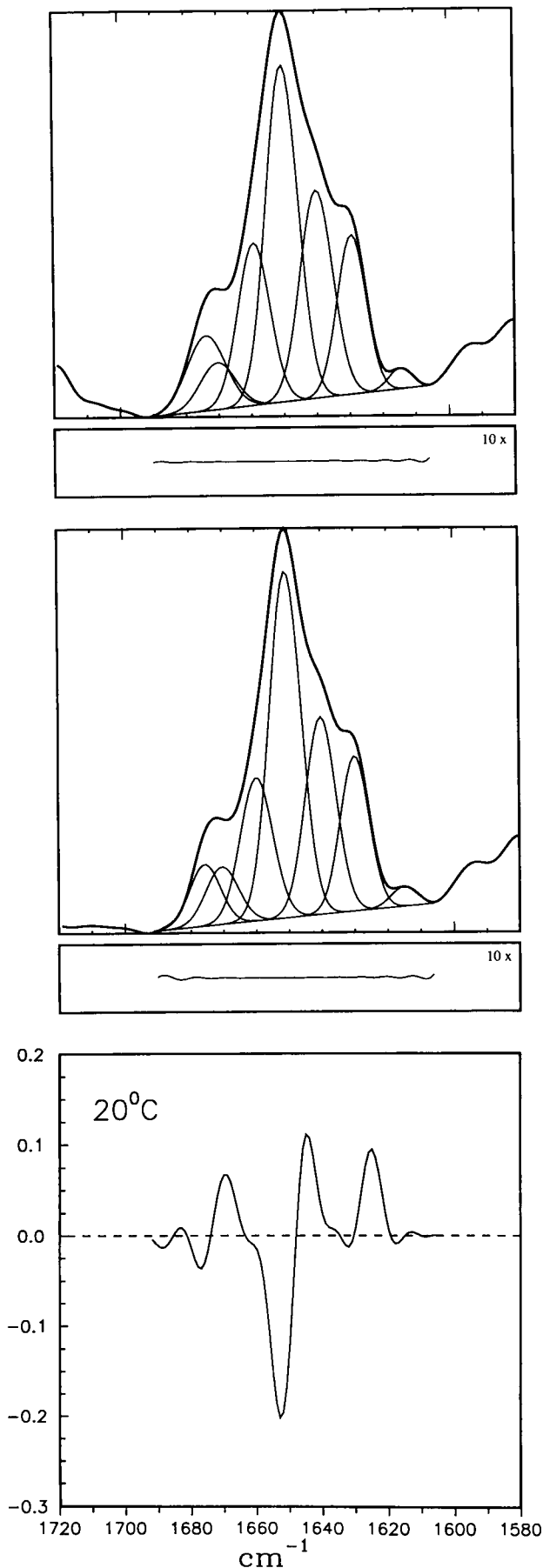
FIGURE 1 Fourier self-deconvoluted FTIR spectra (amide I region) of cytochrome c bound to dimyristoyl phosphatidylglycerol ( upper ) and of cytochrome c in solution ( middle ), at 20°C. Band fitting and residuals ( \times 10 ) obtained by using Gaussian line profiles and the parameters given in Table 1 are shown. The difference between the two upper spectra (with lipid minus without lipid), where the area of each is normalized to 100\text{ cm}^{-1} , is given in the lower panel.
