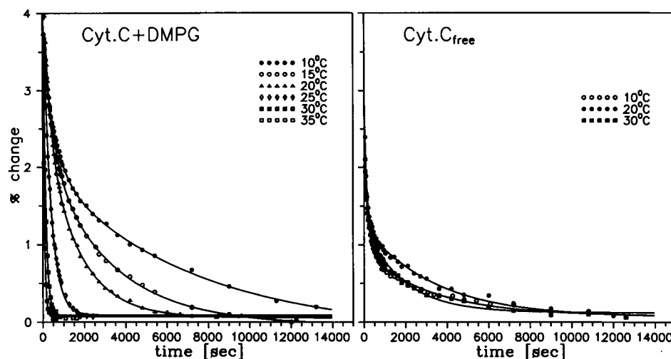
FIGURE 7 Dependence on time after dispersion in D 2 O of the area above the baseline in the FTIR difference spectra (amide I region) of cytochrome c complexed with DMPG (left) and of cytochrome c in solution (right). Difference spectra were obtained by subtracting the FTIR spectrum recorded after extensive deuteration (see Fig. 6). The time courses of deuteration were recorded at the temperatures indicated.
